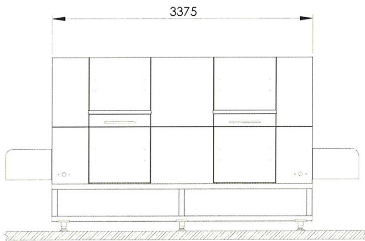
MODEL NPS-F4 (1000 CRATES / HOUR CAPACITY)
