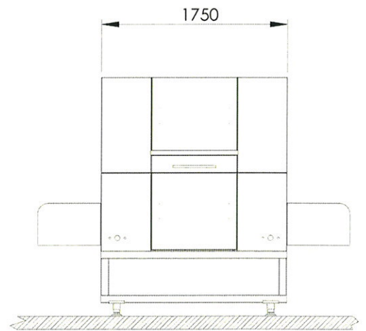
MODEL NPS-F2 (500 CRATES / HOUR CAPACITY)
